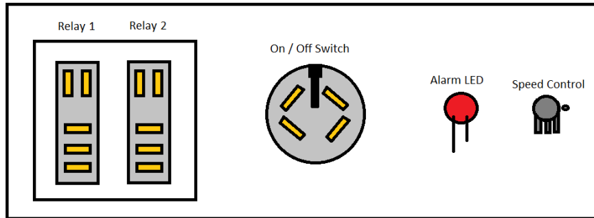
View from inside the electrical compartment
